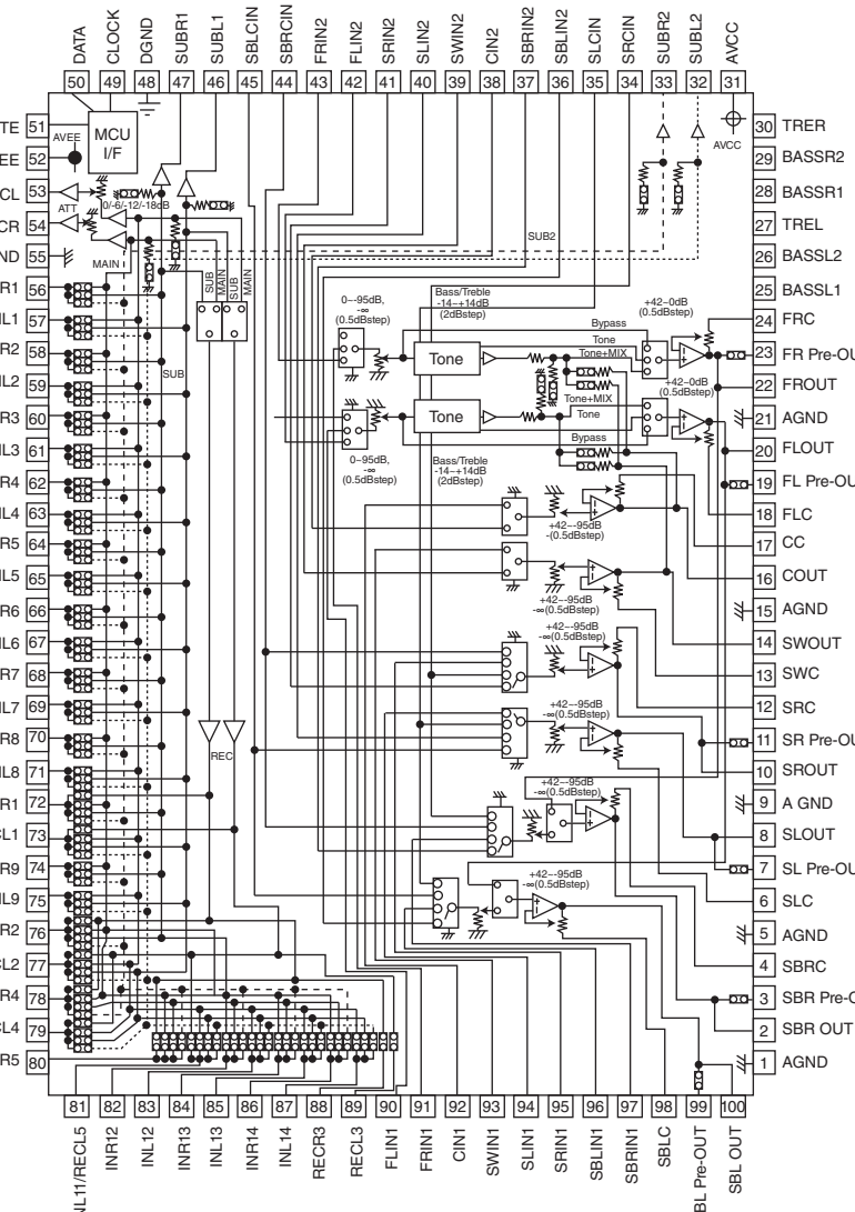
IC741, 742: R2A15220FP 8-channel electronic volume with 11 input selector and tone control
