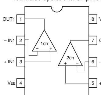
IC763: BA15218F Dual high slew rate, low noise operational amplifier
