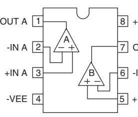
IC724, 726-728: LM833MX Operational amplifier
