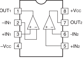
IC701: NJM2068MD-TE2 Dual operational amplifier
