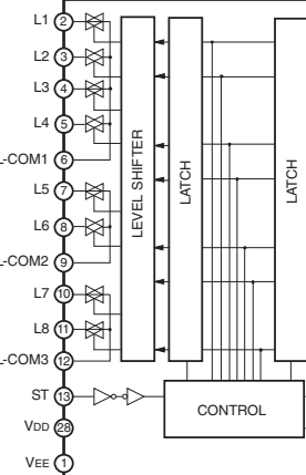
IC743: NJU7313AM Analog function switch
